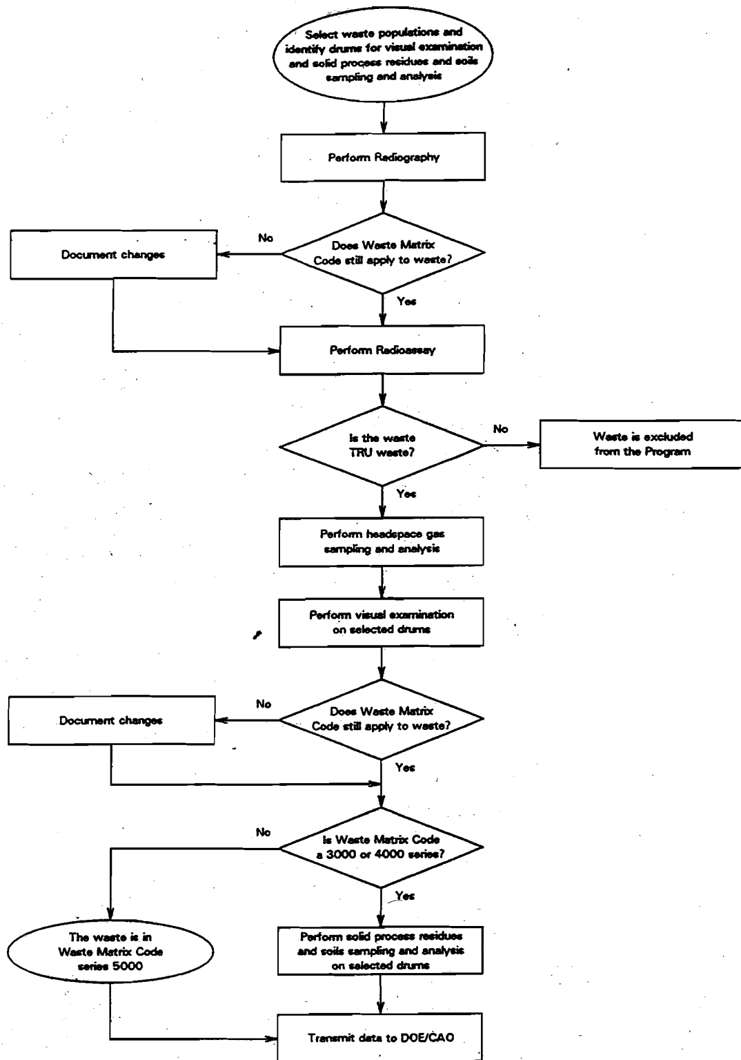
Figure 4-1. Generalized Sequence for TRU Waste Characterization
