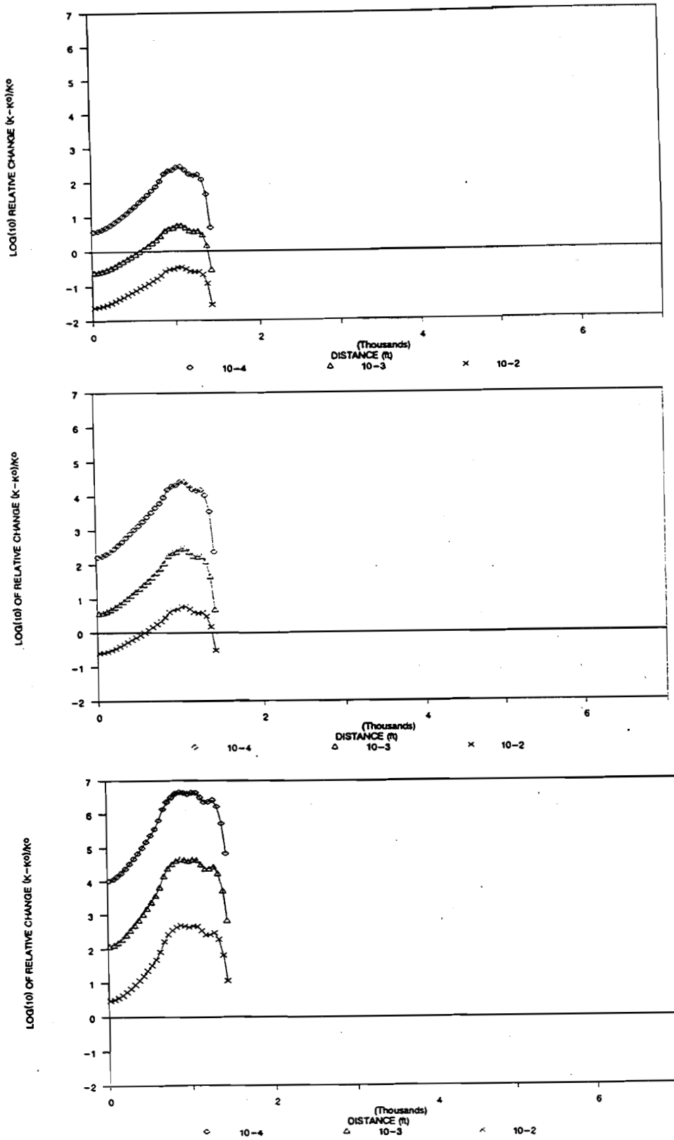
Figure 9-17. Relative Change in Fracture Hydraulic Conductivity for Horizontal Joints with various Fracture Spacings, Subsidence Factor of 67.5%, and Fracture Apertures of 10^{-4} , 10^{-3} , and 10^{-2} in. a) 3 inch b) 30 inch c) 300 inch
