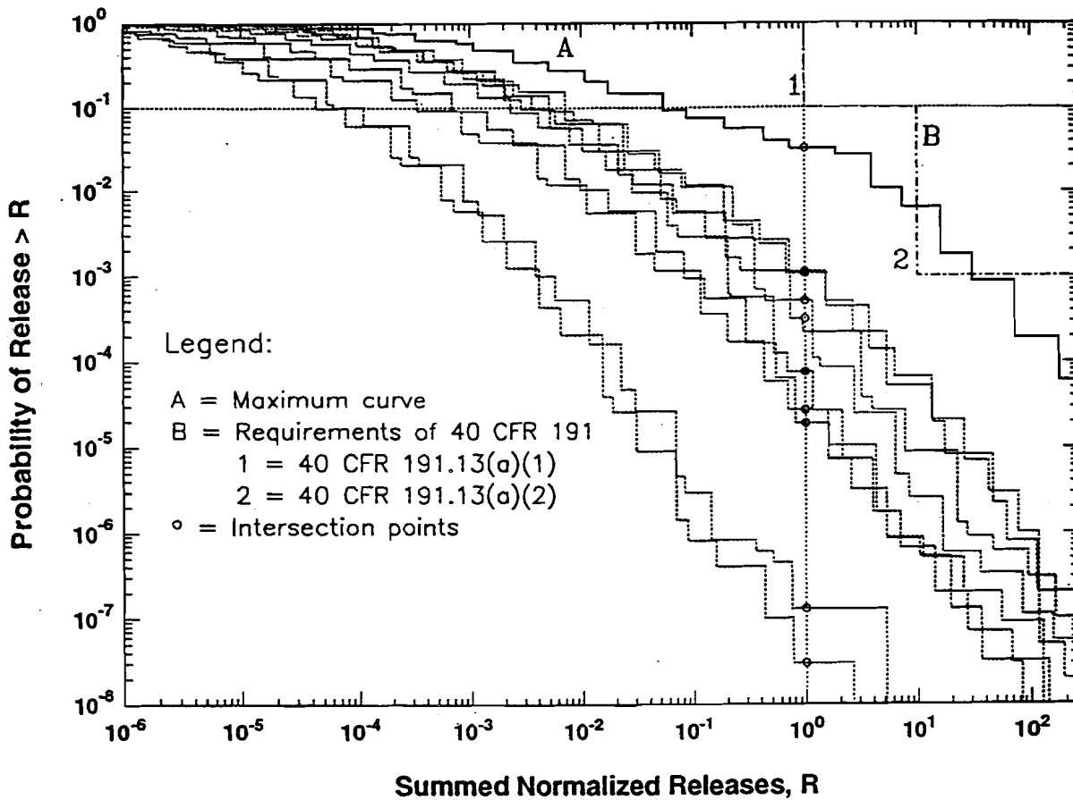
Figure 8-1. Ten Hypothetical LHS CCDFs, with Maximum
